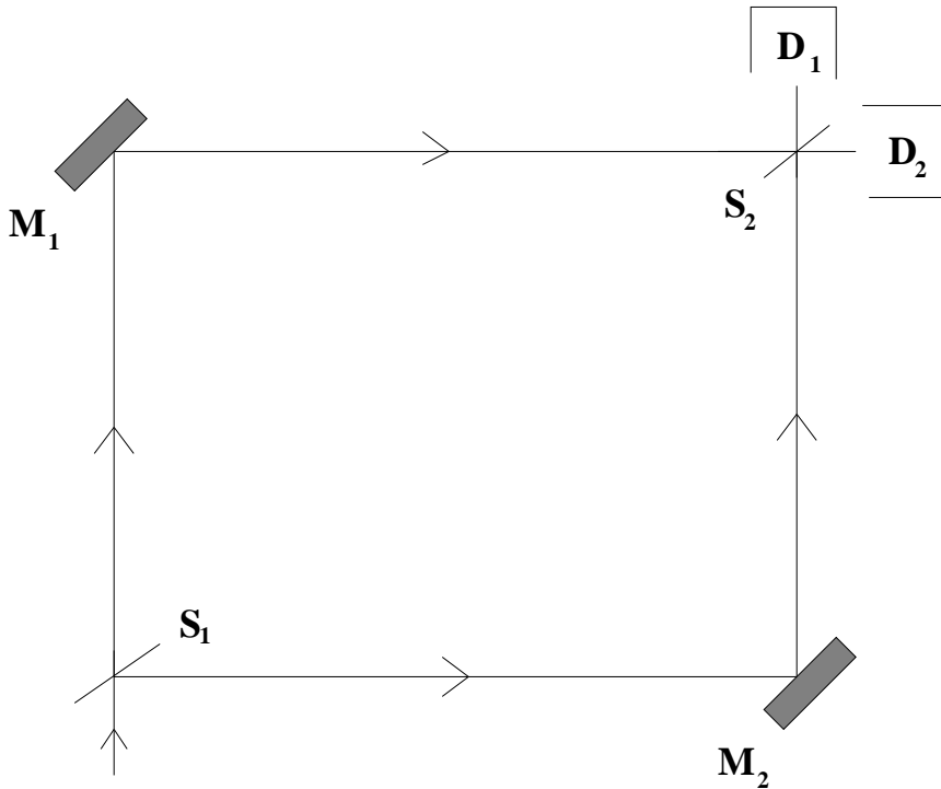
Figure 1. A simple interferometer where a particle enters as indicated and encounters a beam splitter ( S_1 ), a mirror ( M_1 or M_2 ), a second beam splitter ( S_2 ) ending up either in detector D_1 or in detector D_2 .
