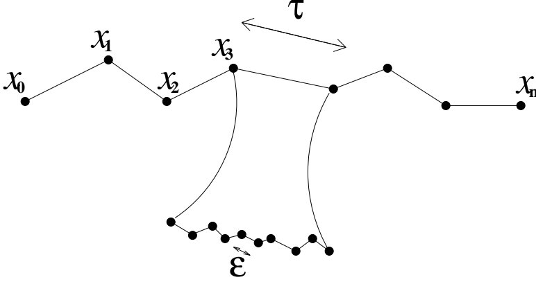
Figure 3. For x_0, x_n \in U , the complex probability ( x_0 \rightarrow x_n ) is equal to a “path integral” over x_1, x_2, \dots, x_{n-1} with time step \tau . The argument can be repeated making n sub-path integrals with time step \epsilon .
