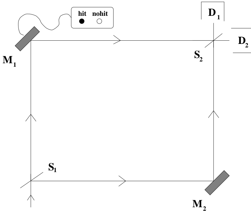
Figure 2. A interferometer similar to the one shown in figure 1. The device is attached to the mirror M_1 records whether M_1 was struck by the particle or not.
